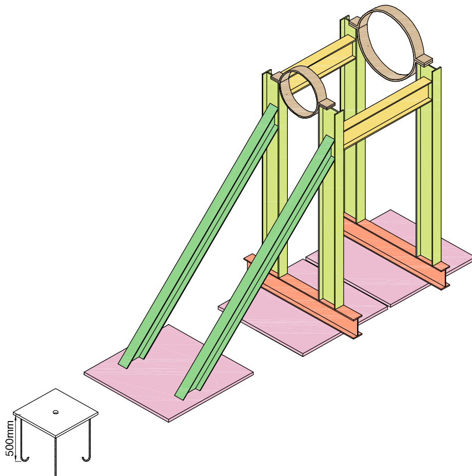
PLACA 500x500x15mm 4 Ø12mm DE 500mm
